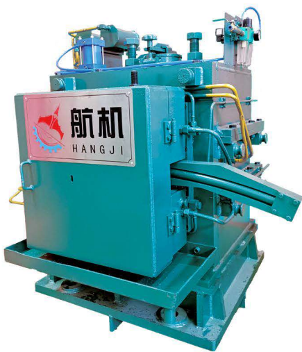
90 m/135 m High speed pinch roll
